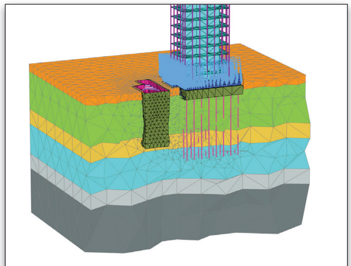
Excavation next to a building on a pile raft foundation.
